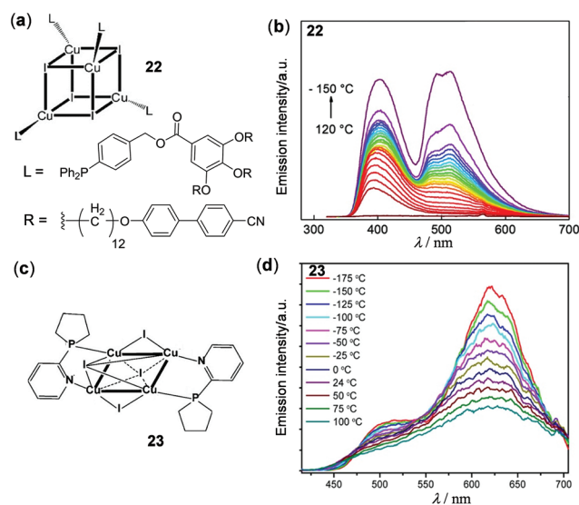
Fig. 20 (a) Chemical structure of the cubane-like Cu 4 -I 4 cluster 22 . (b) Temperature-dependent emission spectra of 22 within the temperature range between -150 and 120 °C (λ ex = 280 nm). Reprinted with permission from ref. 116. Copyright 2016 American Chemical Society. (c) Chemical structure of the octahedral Cu 4 -I 4 cluster 23 . (d) Temperature-dependent emission spectra of 23 recorded from -175 to 100 °C. Reprinted with permission from ref. 117. Copyright 2019 American Chemical Society.
