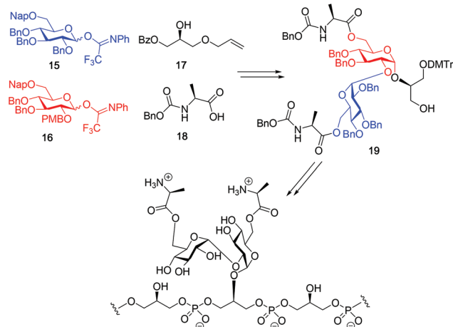
Scheme 3 Building blocks applied in the here-presented studies in the synthesis of D-alanine kojibiose functionalized LTA-fragments of Enterococcus faecalis .
