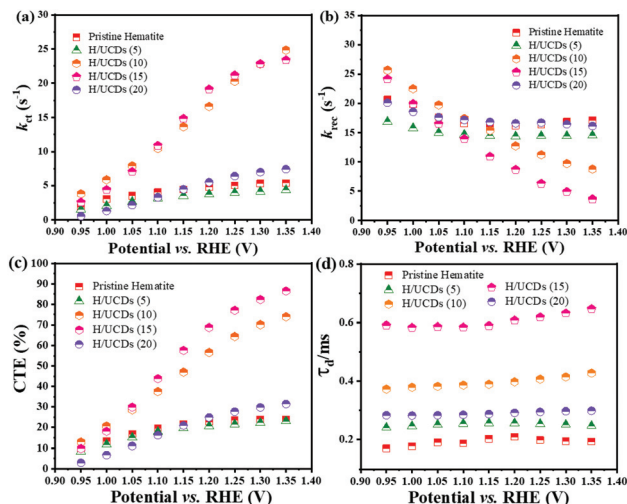
Fig. 7 (a) k_{\text{tr}} , (b) k_{\text{rec}} , (c) charge transfer efficiency (CTE), and (d) diffusion lifetime of the photogenerated charge carriers calculated from IMPS plots.
