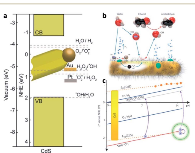
Fig. 16 Experimental energy band alignments for photocatalytic applications of CdS NR/M HNSs. (a) CdS NR (CB and VB) with either Au or Pt tips ( E_F ) and the relevant HER, OER and intermediate radical energy positions on the electrochemical normal hydrogen electrode (NHE) and absolute vacuum scales. Reproduced with permission from ref. 348, Wiley-VCH Verlag GmbH & Co., copyright 2018. (b) Schematic reaction of the CdS NR/Ni photocatalyst producing H 2 (g) (HER) and oxidizing EtOH using a hydroxide intermediate, (c) the corresponding energy scale (y axis) of these reactions as a function of pH (x axis); reproduced with permission from ref. 69, Springer Nature publishing group, copyright 2014.
