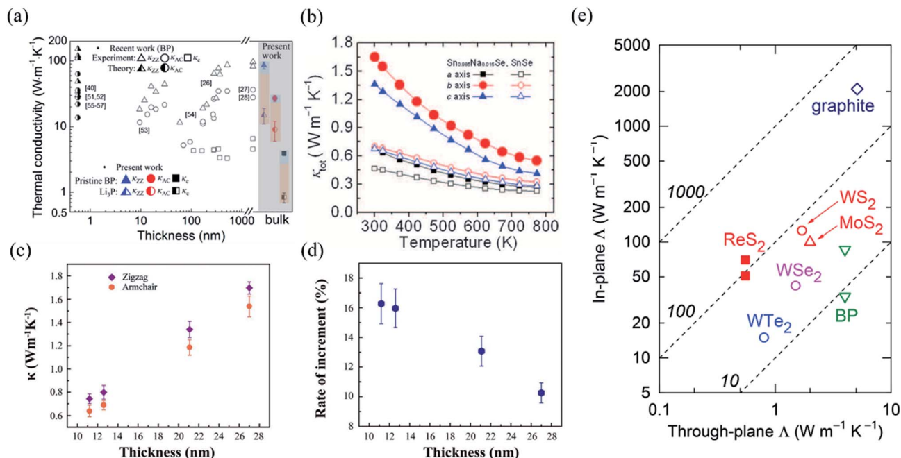
Fig. 16 (a) Summarization of thermal conductivity measurement in three different directions plotted in comparison to the reported values as a function of thickness. Thermal conductivities of black phosphorus for the zigzag (blue), the armchair (red), and cross-plane (black) are shown to illustrate the thermal regulation range from the fully charged state (filled symbols) to the fully discharged state (half-filled symbols). Reproduced from ref. 178 with permission from American Chemical Society. (b) Total thermal conductivity as a function of temperature for SnSe crystals. Reproduced from ref. 14 with permission from American Association for the Advancement of Science. (c) The extracted thermal conductivities along the zigzag and armchair directions of Td-WTe 2 with different thicknesses. (d) The anisotropic difference in thermal conductivities as a function of sample thickness. Reproduced from ref. 181 with permission from Wiley-VCH. (e) Thermal conductivity of 2D materials whose in-plane and through-plane thermal conductivities in the bulk limit have been experimentally determined at room temperature. The data are taken from graphite, 184 MoS 2 , 183 WS 2 , 185 WSe 2 , 186 WTe 2 , 187 and BP. 177 The dashed lines represent constant anisotropy ratio (i.e., the in-plane to through-plane thermal conductivity ratio). 182 Reproduced from ref. 182 with permission from Wiley-VCH.
