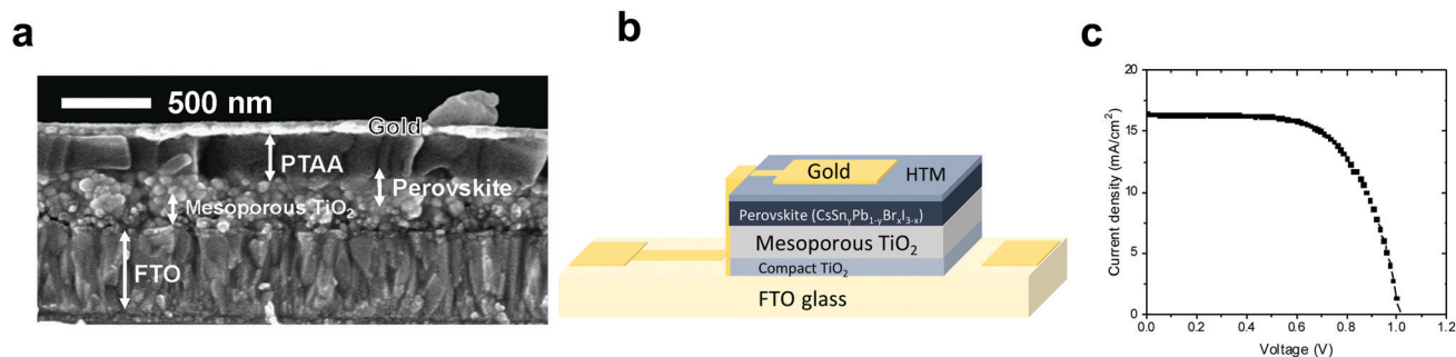
Fig. 6 (a) Cross section SEM image of the PSC with a ratio of 80 : 20 ( \text{CsSn}_{0.2}\text{Pb}_{0.8}\text{I}_{2.6}\text{Br}_{0.4} ) (Pb : Sn) and PTAA as the HTM. (b) Schematic illustration of the perovskite solar cell configuration used in this work. (c) JV curve of the champion cell presenting 12.7% efficiency, a FF of 64.2%, a J_{\text{sc}} of 19.09 \text{ mA cm}^{-2} and a V_{\text{oc}} of 1 V.
