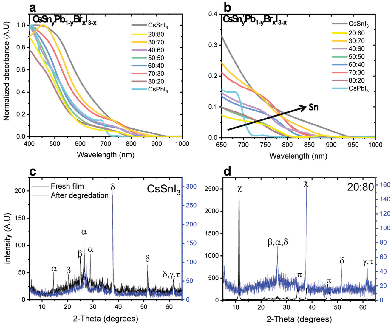
Fig. 1 (a) Absorbance spectra of \text{CsSn}_y\text{Pb}_{1-y}\text{Br}_x\text{I}_{3-x} ( 0 \leq y \leq 1 , 0 \leq x \leq 3 ) films encapsulated at different ratios of \text{Pb}:\text{Sn} . (b) Magnification of the absorbance spectra (shown in (a)) in the range of 650–1000 nm. XRD patterns of (c) \text{CsSnI}_3 and (d) \text{CsSn}_{0.8}\text{Pb}_{0.2}\text{Br}_{1.4}\text{I}_{1.6} ( \text{Pb}:\text{Sn} = 20:80 ) before and after degradation. ( \pi – \text{CsPbI}_3 cubic phase, \chi – \text{CsPbI}_3 orthorhombic phase, \alpha – \text{CsSnI}_3 , \delta – \text{SnO}_2 , \beta – \text{SnI}_2 , \gamma – \text{PbI}_2 , \tau – \text{CsI} .)
