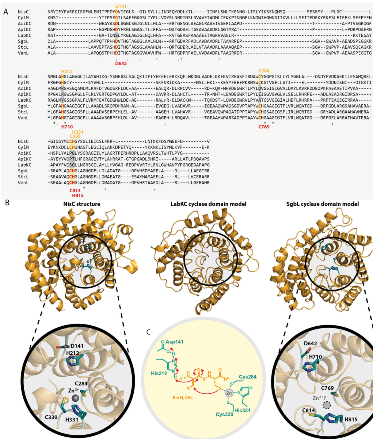
Fig. 7 (A) Excerpt of an alignment of the NisC cyclase (involved in the biosynthesis of the class I lanthipeptide nisin) and the Cy1M cyclase domain (involved in the biosynthesis of the class II cytolysin lanthipeptides) with the cyclase domains of exemplary class III (Ac1KC, Ap1KC, LabKC) and class IV (Sgbl, StcL, VenL) lanthipeptide synthetases. Catalytic residues of class I and II cyclases are highlighted in orange, catalytic residues of the class IV cyclase domains in red. Above the alignment, numbering of the catalytic residues of NisC are shown. Below the alignment, numbering of the predicted catalytic residues of Sgbl are shown. (B) Comparison of the crystal structure of NisC (PDB code 2G0D) with the Phyre2 models of the LabKC and Sgbl cyclase domains. Close ups of the active site of NisC and the predicted active site of the Sgbl cyclase domain are shown. Catalytic residues are highlighted in teal. (C) Schematic showing the catalyzed cyclization reaction with the hypothesized 2,5,68,69 functions for the catalytically important residues in NisC.
