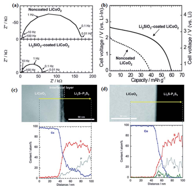
Fig. 11 (a) Impedance profiles of the all-solid-state cells \text{In}/\text{Li}_2\text{S-P}_2\text{S}_5 with solid electrolyte non-coated and \text{Li}_2\text{SiO}_3 -coated \text{LiCoO}_2 at -30^\circ\text{C} after charging to 3.6 V vs. \text{Li}/\text{Li-In} . (b) Discharge curves of the all-solid state cells under the current density of 0.064 \text{ mA cm}^{-2} at 30^\circ\text{C} . (c) Cross-sectional HAADF-STEM image of \text{LiCoO}_2 electrode/ \text{Li}_2\text{S-P}_2\text{S}_5 solid electrolyte interface after initial charging and cross-sectional EDX line profiles for Co, P, and S elements. (d) Cross-sectional HAADF-STEM image of the \text{Li}_2\text{SiO}_3 -coated \text{LiCoO}_2 / \text{Li}_2\text{S-P}_2\text{S}_5 interface after initial charging and cross-sectional EDX line profiles for Co, P, S, and Si elements. 99,108 Reproduced with permission. Copyright© (2009, 2010), American Chemical Society.
