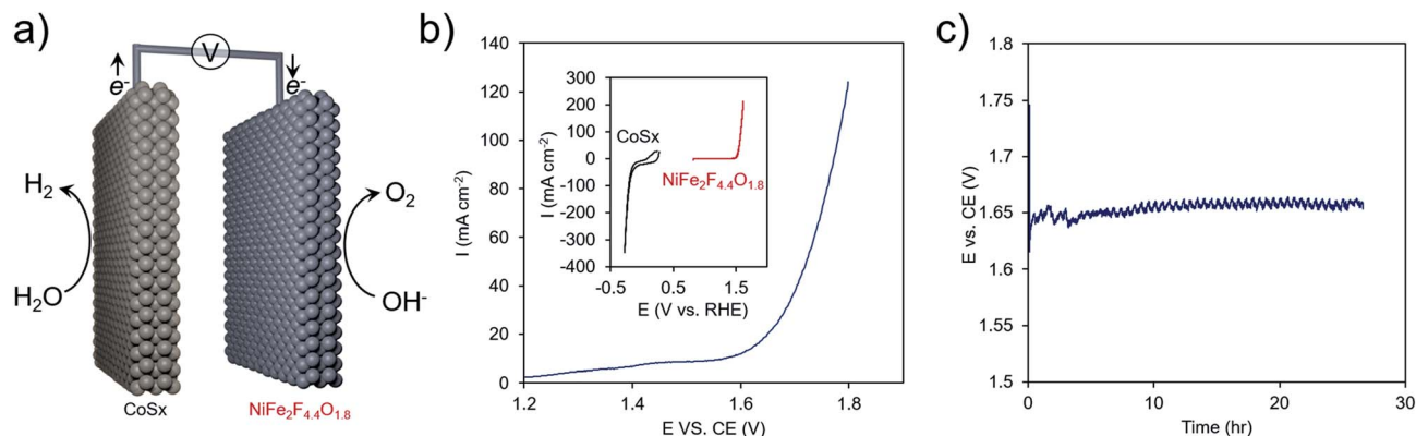
Fig. 8 (a) Overall water electrolysis with \text{NiFe}_2\text{F}_{4.4}\text{O}_{1.8} as the anode. (b) A \text{NiFe}_2\text{F}_{4.4}\text{O}_{1.8} was integrated with a \text{CoS}_x cathode to put together an overall water electrolysis system comprised of earth-abundant materials. (c) This system featured an onset of \sim 1.60 V and required \sim 1.65 V to generate a stable current of 10 \text{ mA cm}^{-2} .
