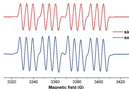
Fig. 19 EPR spectrum of radical anion [(^{Cy}cAAC)Si(P-Tip)]_2^{\cdot-} ( 64 ·- ) in toluene at 285 K.
