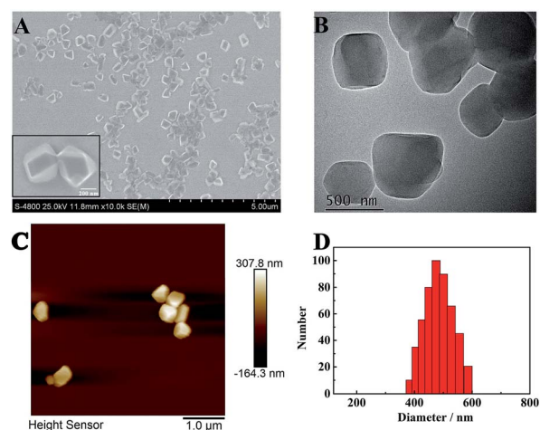
Fig. 1 (A) SEM, (B) TEM, and (C) AFM images, and (D) size distribution of the TPE NCs.
