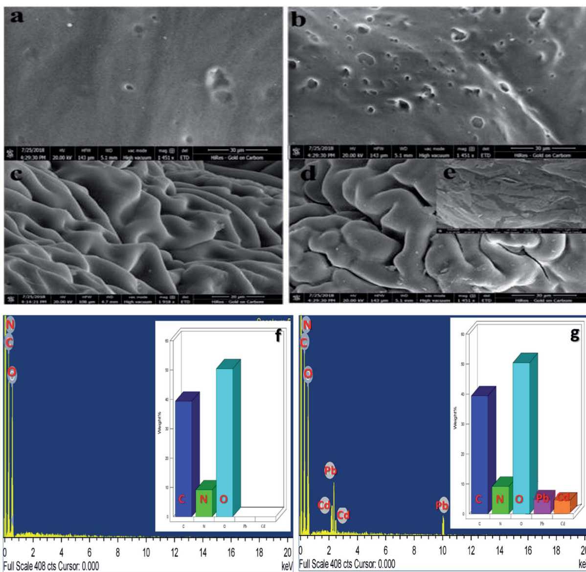
Fig. 3 SEM micrographs of (a) CS, (b) CM, (c) CS-ag-CM, (d) Pb(II)/Cd(II)-CS-ag-CM (e) Pb(II)/Cd(II)-CS-ag-CM and EDX spectrum of (f) CS-ag-CM and (g) Pb(II)/Cd(II)-CS-ag-CM.
