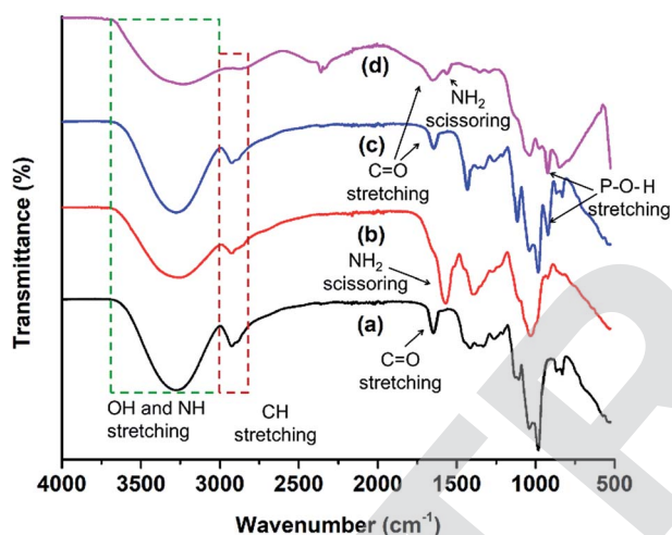
Fig. 2 FTIR spectral analysis of (a) MCDs, (b) N-doped MCDs, (c) P-doped MCDs and (d) dual-doped MCDs.
