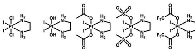
Fig. 1 First-generation photoactive diiodo-Pt(IV) complexes.
