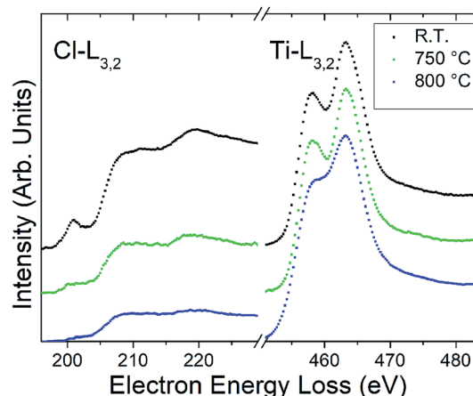
Fig. 4 Electron energy loss spectroscopy from a thin edge of a \text{Ti}_3\text{C}_2\text{T}_2 multilayer particle, showing the background subtracted and multiple scattering deconvolved Cl- and Ti-L 3,2 edges under ambient conditions and after heating at 750 and 800^\circ\text{C} . The spectra are normalized against the Ti-L 2 peak maximum and vertically separated for clarity.
