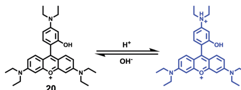
Scheme 15 Fluorescent probe 20 for pH.
