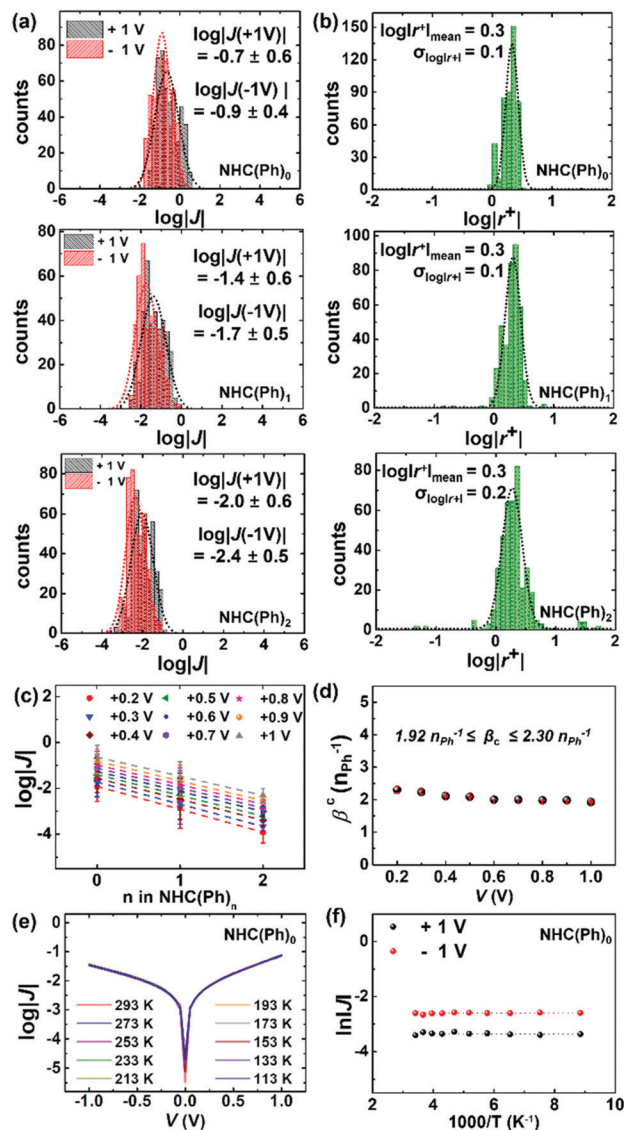
Fig. 2 Histograms of (a) \log|J| and (b) \log|r^{\pm}| at ±1.0 V for NHC(Ph) n ( n = 0, 1, and 2) SAM. (c) Linear correlation between the \log|J| and the molecular length. (d) Constant \beta^c value regardless of applied voltage. (e) Exemplary \log|J| – V traces measured at low temperatures (from 113 to 293 K) for Au TS /NHC(Ph) n //Ga 2 O 3 /EGaIn junctions. (f) The corresponding Arrhenius plots.
