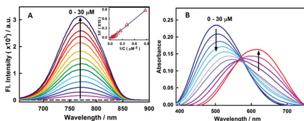
Fig. 1 (A) Fluorescence spectra of 15 \mu\text{M} styryl-11 with increasing concentration of insulin fibrils (0– 30 \mu\text{M} ) [ \lambda_{\text{ex}} = 630 nm]. Inset shows the double reciprocal plot ( 1/F vs. 1/C ) and the solid line represents the fitting of the data points according to the 1:1 binding model. (B) Absorption spectra of 15 \mu\text{M} styryl-11 with the increase in concentration of insulin fibrils (0– 30 \mu\text{M} ).
