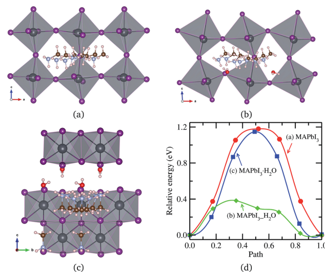
Fig. 5 MA + ion migration in (a) pseudo-cubic MAPbI 3 , (b) water intercalated phase MAPbI 3 ·H 2 O and (c) monohydrated phase MAPbI 3 ·H 2 O, and (d) corresponding activation energy profile.
