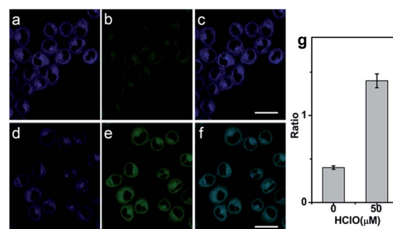
Fig. 2 TP images of exogenous HClO with QC10 in HeLa cells. HeLa cells were treated with 5.0 \mu\text{M} QC10 for 0.5 h (a, b, and c) and then with 50 \mu\text{M} HClO for 0.5 h (d, e, and f). (g) Fluorescence intensity ratios from overlay images of (c) and (f). The fluorescence intensities were collected at the blue channel (400–500 nm) and the green channel (550–600 nm) respectively upon two-photon excitation at 820 nm. Scale bar: 20 \mu\text{m} . Incubation time: 0.5 h.
