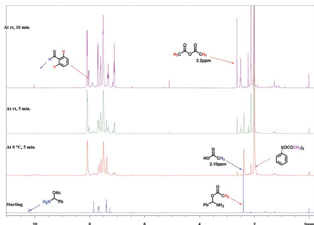
Fig. 2 Time dependent 1 H NMR experiment for mechanistic determination on intermediate.
