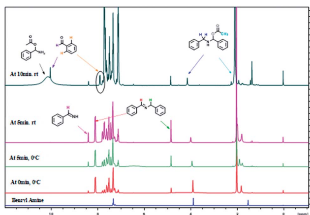
Fig. 1 Time dependent 1 H NMR experiment for mechanistic determination.
