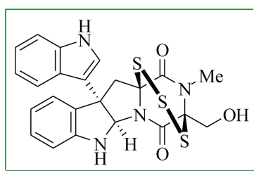
Scheme 152 Total synthesis of (+)-luteoalbusin A 704 and (+)-luteoalbusin B 705.
