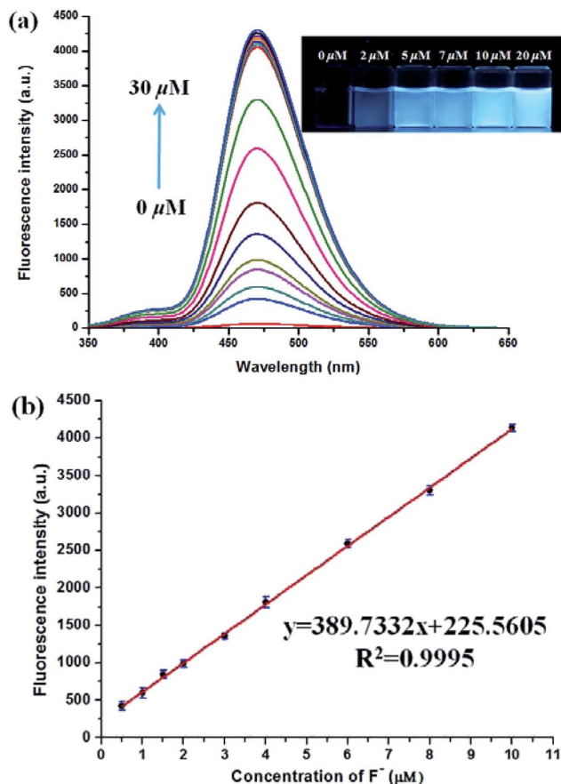
Fig. 4 (a) The fluorescence spectra of PBT in the presence of different concentrations of F^- [PBT is 10 \mu M ], [Tris buffer is 20 \text{ mM} ] in a mixture of THF and Tris buffer solution (pH 8.0), (1 : 9, v/v), \lambda_{\text{ex}} = 335 \text{ nm} , \lambda_{\text{em}} = 470 \text{ nm} . Inset: direct observation of the difference in fluorescence intensity of PBT under UV irradiation (365 nm) with various concentration F^- (0–20 \mu M ) after 10 min incubation time. (b) The linear relationship between fluorescence intensity and F^- concentration (0.5–10 \mu M ).
