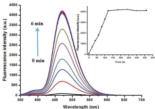
Fig. 5 Time course of the signaling of PBT by F^- [PBT is 10 \mu M ], [ F^- is 20 \mu M ], in a mixture of THF and Tris buffer solution (pH 8.0), (1 : 9, v/v), \lambda_{\text{ex}} = 335 \text{ nm} , \lambda_{\text{em}} = 470 \text{ nm} . Inset: the response curve of fluorescence intensity of PBT with F^- depending on the various time.
