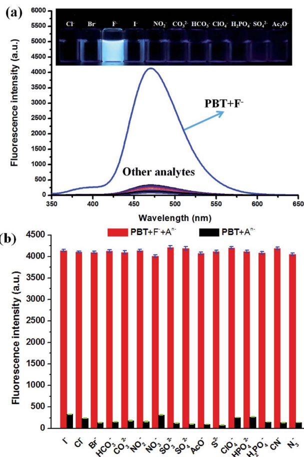
Fig. 6 (a) Fluorescence spectra of PBT in the presence of various anions. [PBT] = 10 \mu M , [ An^- ] = 20 \mu M , in a mixture of THF and Tris buffer solution (pH 8.0), (1 : 9, v/v), \lambda_{\text{ex}} = 335 \text{ nm} , \lambda_{\text{em}} = 470 \text{ nm} . Inset: direct observation of fluorescence emission difference of the probe PBT ( 10 \mu M ) under UV irradiation (365 nm) in the presence of different anions. Left to right: Cl^- , Br^- , I^- , F^- , NO_2^- , CO_3^{2-} , HCO_3^- , ClO_4^- , H_2PO_4^- , SO_4^{2-} and AcO^- . (b) The selectivity of PBT in the presence of various anions.
