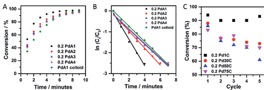
Fig. 4 (A) Conversion profiles of Pd catalysts for the hydrogenation of p -nitrophenol, (B) \ln(C_t/C_0) versus time plots for Pd catalysts tested for p -nitrophenol and (C) catalyst recycling studies outlining the conversion achieved through five successive cycles of p -nitrophenol hydrogenation over each 0.2 wt% Pd/TiO 2 catalyst, conversion calculated after 5 minutes. Reaction conditions: p -nitrophenol : Pd molar ratio = 13, NaBH 4 : p -nitrophenol molar ratio = 24.
