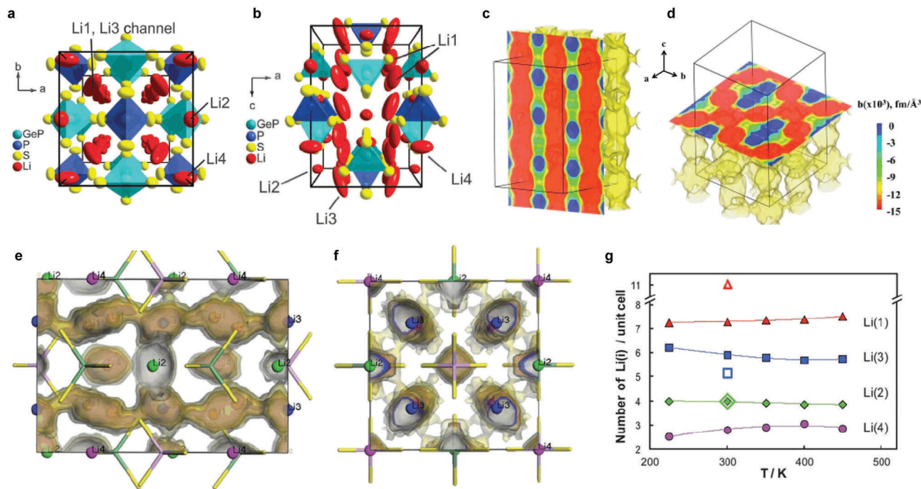
Fig. 7 (a and b) Unit cell of tetragonal \text{Li}_{10}\text{GeP}_2\text{S}_{12} with thermal ellipsoids ( \rho = 0.8 ); 219 Reproduced with permission from ref. 219. Copyright (2013) the Royal Society of Chemistry. (c) MEM reconstructed negative nuclear density maps in \text{Li}_{10}\text{GeP}_2\text{S}_{12} (surface threshold -0.015 \text{ fm} \text{ \AA}^{-3} , cell grid 256 \times 256 \times 512 ) and slices in (c) (011) and (d) (001) planes, respectively; (d) shows the diffusion tunnels within \text{Li}_{10}\text{GeP}_2\text{S}_{12} along the \langle 001 \rangle direction, whereas the Li distribution along (110) can be seen in (d); 220 Reproduced with permission from ref. 220. Copyright (2016) American Chemical Society. (e and f) Li distribution from a 10 ns NVT MD simulation of a 3 \times 3 \times 2 supercell at T = 300 \text{ K} projected into a single unit cell (shown (e) along [100] and (f) along [001]). Regions of highest Li density (darkest isosurface) coincide with the 4 Li sites, the easiest path for transport (lighter isosurface) corresponds to the Li(3)–Li(1) channels along [001]. The lightest isosurface reveals a significant probability for hops Li(3)–Li(2) establishing a 3D network of pathways. With a lower probability, Li(4) sites are attached to this pathway network (not shown); 218 (g) temperature dependence of Li distribution on the four Li sites identified by MD simulations (filled symbols). The corresponding open symbols refer to the neutron refinements by Kanno's group, 45 who distributed the 20 Li per unit cell onto Li(1), Li(2) and Li(3) sites only. 218 Reproduced with permission from ref. 218. Copyright (2012) the Royal Society of Chemistry.
