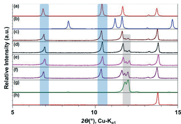
Fig. 2 Simulated pattern of CAF-GLU Form I (monoclinic) (a), simulated pattern of CAF-GLU Form II (triclinic) (b), the ground powder of CAF-GLU as obtained from [\text{C}_2\text{mim}][\text{NTf}_2] (c), [\text{C}_4\text{mim}][\text{NTf}_2] (d), [\text{C}_8\text{mim}][\text{NTf}_2] (e), [\text{C}_{12}\text{mim}][\text{NTf}_2] (f), CAF (g) and GLU (h) used in the grinding experiments.
