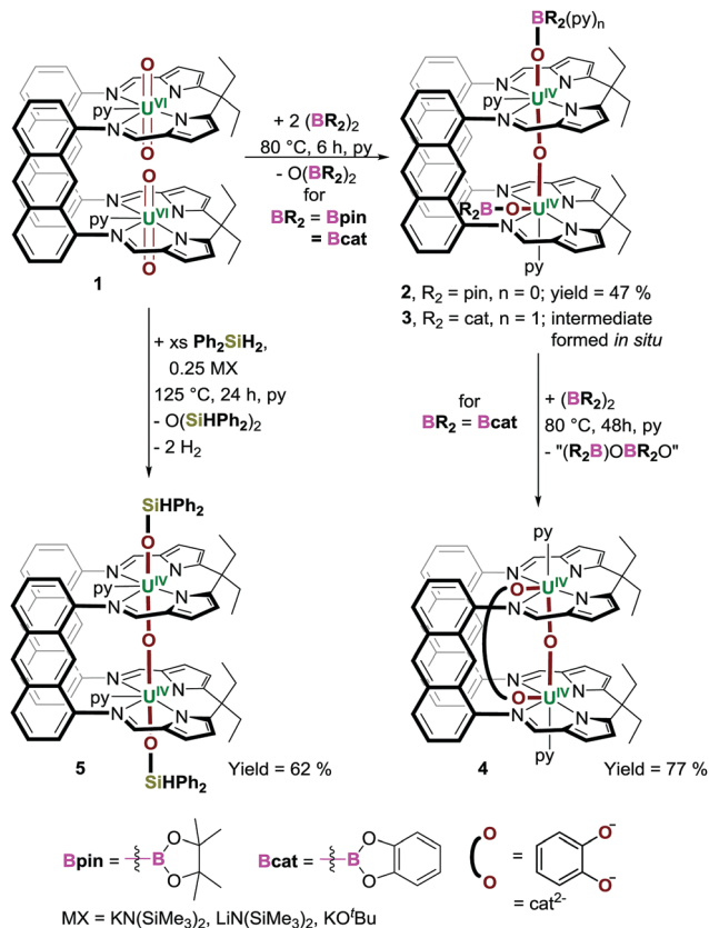
Scheme 1 Diborane or silane-mediated deoxygenation of co-axial uranyl dications to form the new tetracoordination [OUOU] 4+ 2 , 3 , and 5 , with either trans -, cis - (for boron) or trans -, trans - (for silicon) geometry, and the further deoxygenation of 3 to afford the UOU-containing 4 .
