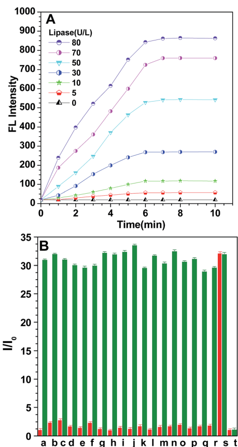
Fig. 2 (A) Time-dependent fluorescence intensity of probe S1 (10 \mu\text{M} ) in hexane solution at 453 nm versus the hydrolysis reaction time in the presence of different concentrations of lipase in PBS (pH 7.4, 0.1 M) at 37 ^{\circ}\text{C} . Excitation wavelength: 360 nm. (B) Fluorescence response of a 10 \mu\text{M} probe in PBS-buffered water (pH 7.4, 0.1 M) at 37 ^{\circ}\text{C} for 15 min in the presence of different biologically-relevant substances (red bars); the fluorescence response of a 10 \mu\text{M} probe in PBS-buffered water (pH 7.4, 0.1 M) at 37 ^{\circ}\text{C} for 15 min in the presence of 80 \text{U L}^{-1} lipase and with the addition of different biological substances respectively (green bars). (a) NaCl; (b) KCl; (c) \text{MgCl}_2 ; (d) \text{CaCl}_2 ; (e) \text{AlCl}_3 ; (f) \text{NaNO}_3 ; (g) \text{Na}_2\text{CO}_3 ; (h) \text{Na}_2\text{SO}_4 ; (i) arginine; (j) leucine; (k) glutamic acid; (l) phenylalanine; (m) cysteine; (n) glucose oxidase; (o) alkaline phosphatase; (p) acylase; (q) laccase; (r) \alpha -amylase; (s) lipase; (t) blank; the concentration of the ions and amino acids is 100 \mu\text{M} , while the concentration of the protein enzymes is 80 \text{U L}^{-1} . Excitation wavelength: 360 nm.
