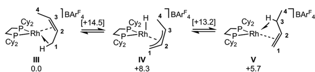
Scheme 12 Computed mechanisms for interconversion of [1-( cis -2-butene)] + , III, and [1-(1-butene)] + , V, cations in the solid-state. Free energies are indicated in kcal mol -1 with those for transition states provided in square brackets.
