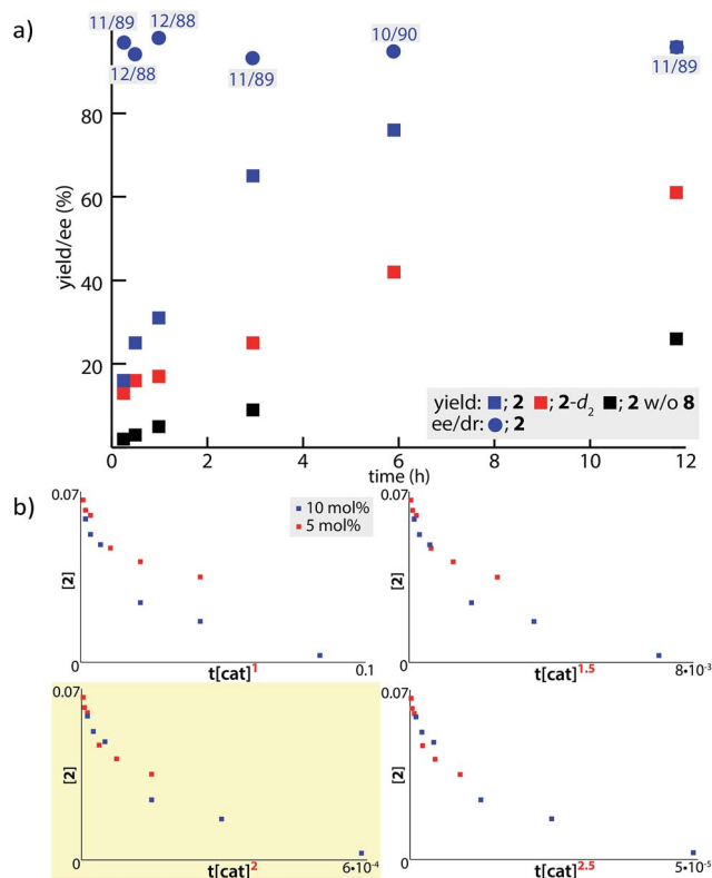
Fig. 2 Kinetic profile of the Cu(II)-catalyzed aldol reaction with 4a . (a) Time course study with 2 (blue) and 2-d 2 (red) from the initial concentration of 70 mM at -60\text{ }^\circ\text{C} . The numbers in grey boxes indicate the diastereomeric ratio of the product ( anti/syn ). The data with black square was obtained from control experiments without ligand 8 . (b) Normalized time scale plots with 5 and 10 mol% catalyst loading.
