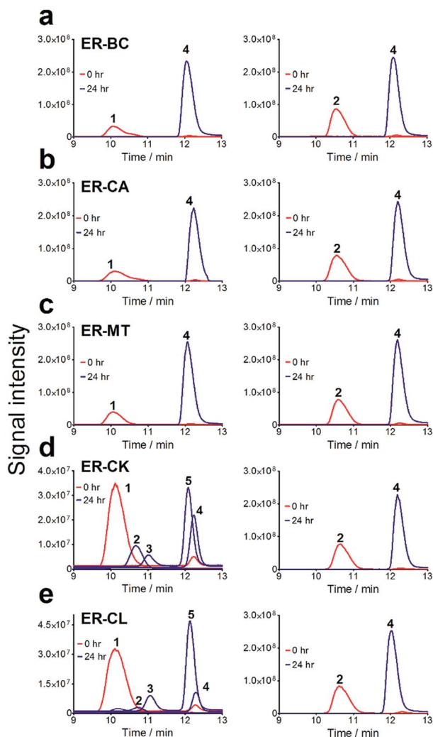
Fig. 2 Biotransformation of cis,cis - and trans,trans -isomers of muonic acid (0.70 mM) by E. coli cells expressing (a) ER-BC, (b) ER-CA, (c) ER-MT, (d) ER-CK, and (e) ER-CL. Substrates and products were detected by LC-MS. (1) cis,cis -muonic acid, (2) trans,trans -muonic acid, (3) 2-hexenedioic acid, (4) adipic acid, and (5) 3-hexenedioic acid-like compound with m/z 143.0319.
