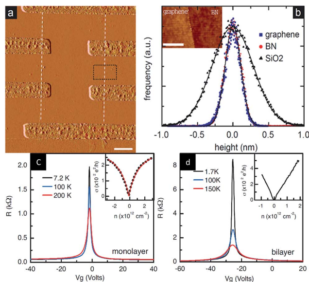
Fig. 37 Graphene/h-BN devices and the test chart. (a) AFM image of graphene/h-BN heterostructure. (b) Histogram of the height distribution measured by AFM for graphene, h-BN and SiO 2 . Resistance versus applied gate voltage for monolayer graphene (c) and bilayer graphene (d) on h-BN. 204
