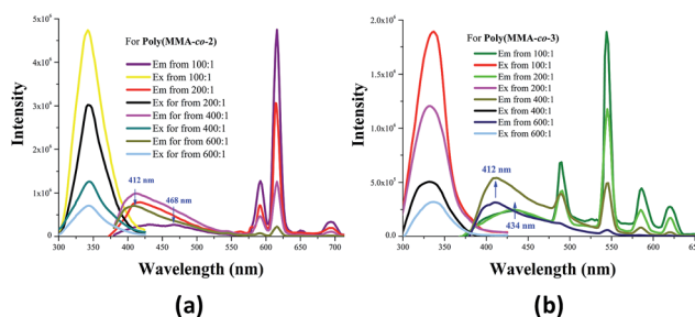
Fig. 6 Emission and excitation spectra ( \lambda_{\text{ex}} = 341 nm) of homo- \text{Ln}^{3+} -grafted polymers with different feed molar ratios (100 : 1, 200 : 1, 400 : 1 and 600 : 1) in the solid state at room temperature; (6a) for Poly(MMA-co-2); (6b) for Poly(MMA-co-3).
