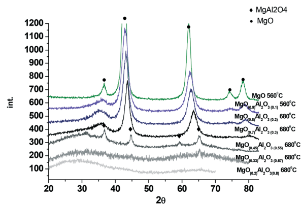
Fig. 2 XRD of the (\text{MgO})_x(\text{Al}_2\text{O}_3)_y samples after calcination at 560^\circ\text{C} or 680^\circ\text{C} .
