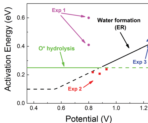
Fig. 5 Predicted activation energies (free energy barriers, \Delta G^\ddagger in eV) for the rate determining steps from QM R \mu D calculations at various applied potentials, compared to experimental data (enthalpy, \Delta H^\ddagger in eV). The theory suggests that \Delta G^\ddagger = 0.25 eV for \text{O}^* hydrolysis (solid green line) is rate determining below 0.87 V, while water formation via ER (solid black line) dominates at higher potential. The potential dependence of water formation (ER) was derived from the simulations at 0.6 V leading to \Delta G^\ddagger = 0.12 eV and at 1.1 V leading to \Delta G^\ddagger = 0.35 eV, leading to a slope of 0.46. The reaction barrier for proton transfer ( \sim 0.1 eV) is taken as the lower limit for this step. The experimental data Exp 2 (red, Paulus et al. 2002) 48 and Exp 3 (blue, Grgur et al. 1997), 46 were determined by fitting to the Arrhenius equation the observed exchange current density (from the Tafel slope) over the temperature range 298–333 K. The results in Exp 1 (purple, Beattie et al. 1999) 45 may involve organic impurities from the Nafion solution. Note that the LH barrier of 0.29 eV for \text{H}^* + *OOH reduction is reduced by the ER mechanism to below the 0.25 eV for \text{O}^* hydrolysis for U > 0 .
