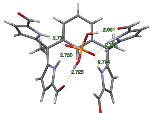
Fig. 4 Single crystal structure of the 1 : 1 complex 4b \cdot \text{H}_2\text{PO}_4^- viewed from the top of the bound \text{H}_2\text{PO}_4^- molecular ion. One \text{TBA}^+ counter cation is associated with each complex. It and a \text{CHCl}_3 solvent molecule are omitted for clarity.
