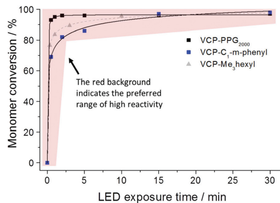
Fig. 3 Determined monomer conversion for the photo-polymerization of VCP-PPG 2000 , VCP- m -phenyl and VCPMe 3 hexyl (1 mol% initiator CQ: EDMAB in a molar ratio of 1:2). The curing was performed under a controlled atmosphere of nitrogen using a commercial LED source (2.013 mW cm -2 for 465 nm).
