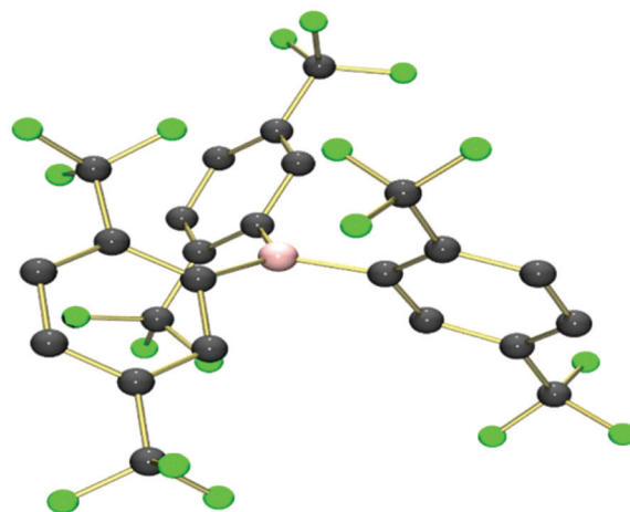
Fig. 2 The crystallographic molecular structure of B\{2,5\text{-}(CF_3)_2C_6H_3\}_3 (hydrogen atoms removed for clarity).
