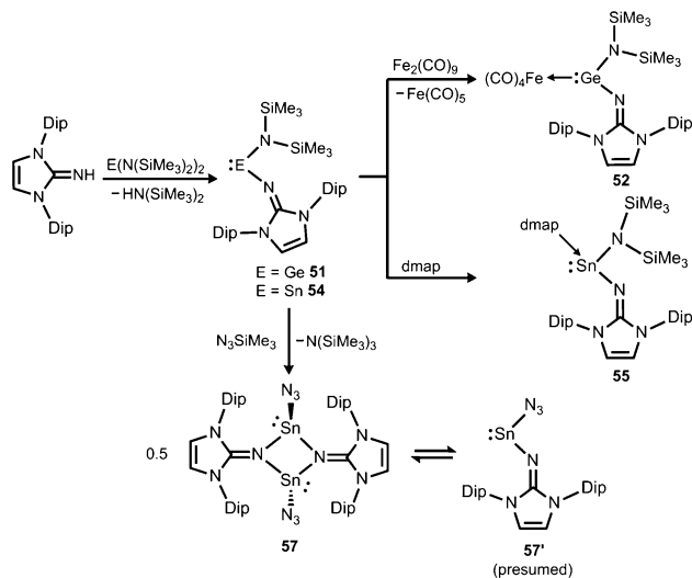
Scheme 12 Preparation of amino(imino)metallylenes 51 and 54 and the iron carbonyl 52 , as well as the dmap adduct 55 ( dmap = 4-dimethylamino-pyridine). Conversion of 54 to dimeric stannylylene azide 57 .
