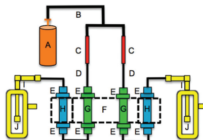
Fig. 1 Schematic of the PFAA gas phase source for dry reactions. A: compressed nitrogen cylinder; B: 1/4" polyethylene tubing; C: Swagelok® VCR assembly; D: 1/8" PFA tubing; E: 1/8-1/2" PTFE union; F: aluminium heating block; G: 1/2" PFA tubing housing acid permeation devices; H: 1/2" PFA tubing housing PFAA salt beds; I: 1/8-1/4" PTFE elbow; J: glass impinger. PFAA salt beds can be placed inside and outside the aluminium heating block. The critical orifice (1 μm pinhole) is housed in C, held between two stainless steel glands.
