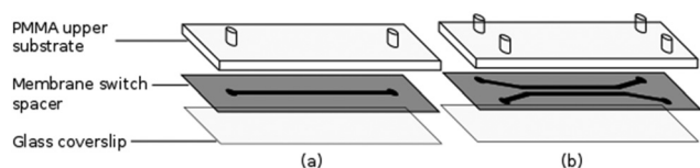
Fig. 2 Construction of (a) single and (b) dual channel devices.
