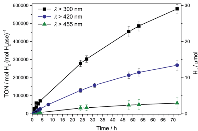
Fig. 2 Photocatalytic H_2 production with Dmb [NiFeSe]- H_2 ase (50 pmol) with CN_x - TiO_2 (5 mg) in EDTA (pH 6, 0.1 M, 3 mL) under AM 1.5G irradiation at an intensity of 1 Sun at \lambda > 300 , 420 and 455 nm.
