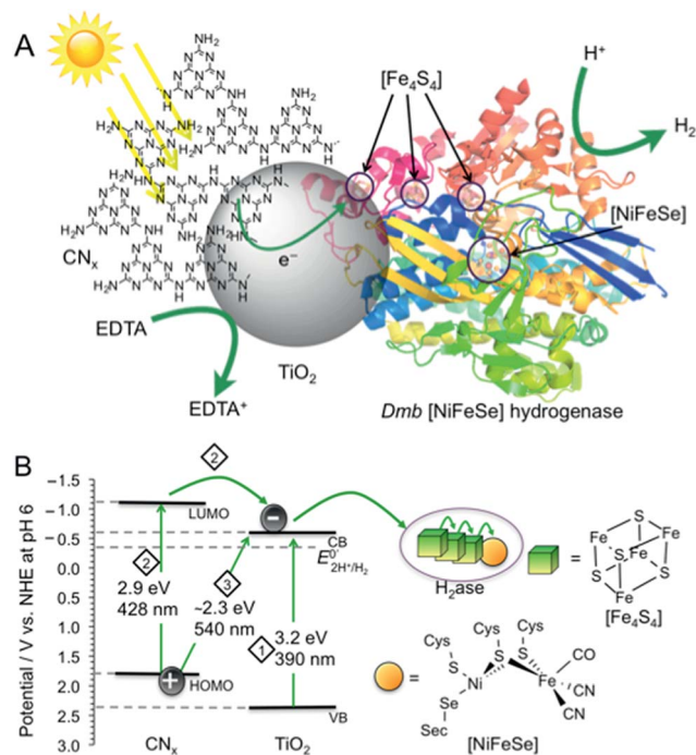
Fig. 1 (A) Schematic representation of photo- H_2 production with Dmb [NiFeSe]- H_2 ase (PDB ID : 1CC1) 14 on CN_x - TiO_2 suspended in water containing EDTA as a hole scavenger. (B) Irradiation of CN_x - TiO_2 can result in photo-induced electron transfer by three distinct pathways: (1) TiO_2 band gap excitation (2) excitation of CN_x ( HOMO_{CN_x} - LUMO_{CN_x} ), followed by electron transfer from LUMO_{CN_x} into the conduction band of TiO_2 ( CB_{TiO_2} ). (3) Charge transfer excitation with direct optical electron transfer from HOMO_{CN_x} to CB_{TiO_2} . The CB_{TiO_2} electrons generated through pathways 1 to 3 are then transferred via the [Fe_4S_4] clusters to the [NiFeSe] H_2 ase active site.
