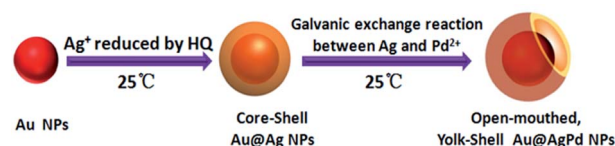
Fig. 1 Schematic representation of the synthetic procedure of open-mouthed, yolk-shell Au@AgPd NPs by galvanic reaction of Au@Ag NPs with \text{Pd}^{2+} ions at room temperature.
