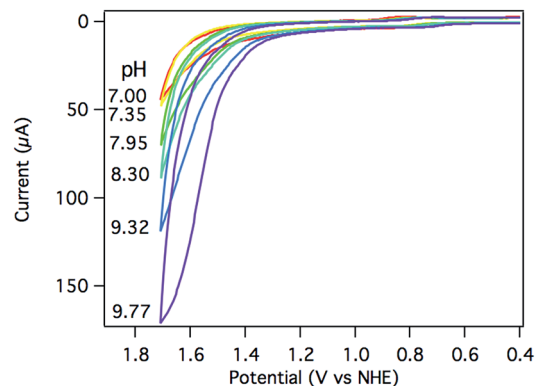
Fig. 5 CV of 0.25 mM [Ru(Py 3 PO)(bpy)(OH 2 )] 2+ at pH 7.00 (red), 7.35 (yellow), 7.95 (green), 8.30 (teal), 9.32 (blue), and 9.77 (purple) at 100 mV s -1 . Conditions: 0.1 M phosphate, 3 mm glassy carbon working electrode, Pt wire counter electrode, Ag/AgCl reference electrode.
