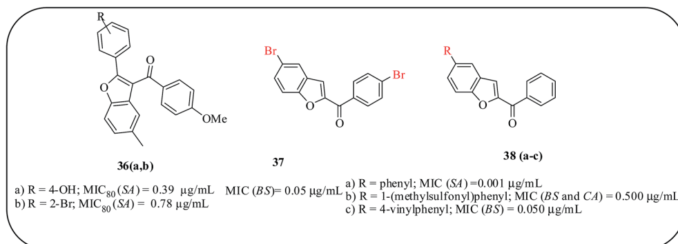
Fig. 10 Structures of phenyl benzofuran derivatives.
