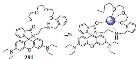
Fig. 255 Chemical structure of ligand 291 and the suggested binding modes of interaction with the metal ions.
