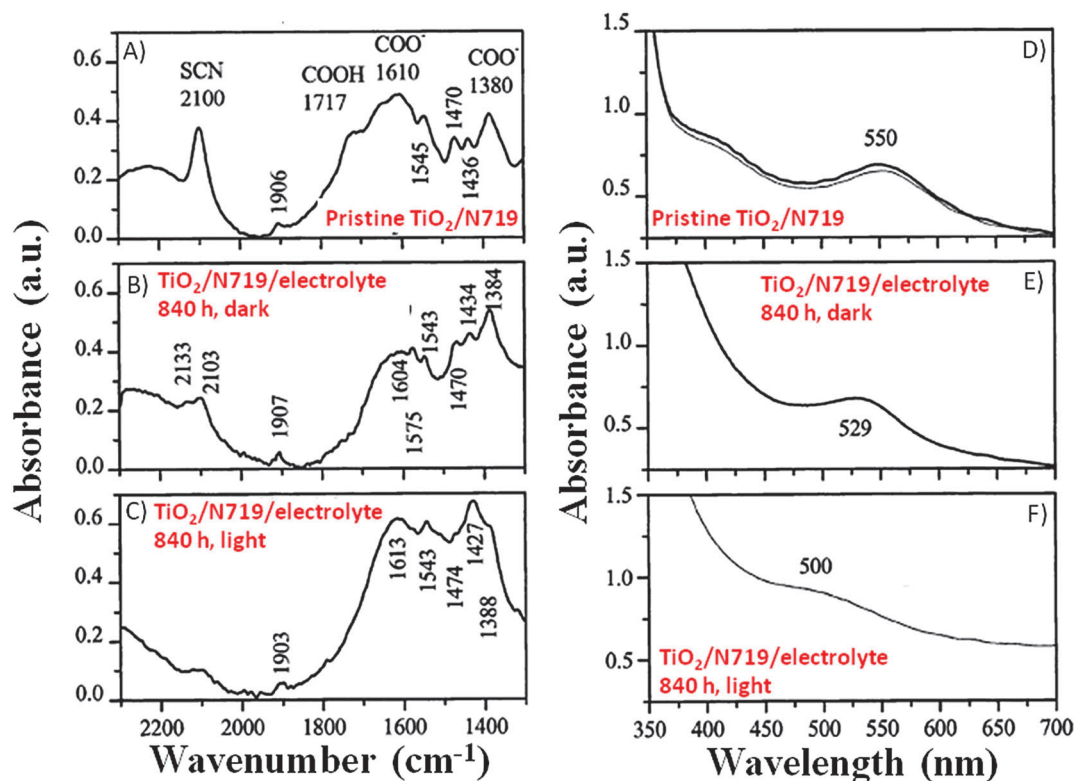
Fig. 4 FTIR (left side) and UV-Vis (right side) spectra of: (A, D) non-treated working electrodes in an Ar atmosphere; (B, E) working electrodes being soaked in a liquid electrolyte (Lil 0.50 M and \text{I}_2 50 mM in MPN) with 5 vol% \text{H}_2\text{O} under dark for 840 h; (C, F) working electrodes being soaked in the same liquid electrolyte under visible light illumination for 840 h. FTIR spectra of the treated samples were normalized based on the \text{TiO}_2 absorption maximum of the reference sample at 832\text{ cm}^{-1} . Adapted and reprinted from ref. 85.
