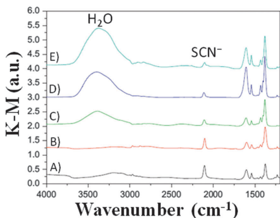
Fig. 5 DRIFT spectra of \text{N719}/\text{TiO}_2 films immersed in liquid electrolytes (Lil 0.50 M, \text{I}_2 50 mM and TBP 0.50 M in ACN) having different water contents for 192 h: (B) 0 vol% \text{H}_2\text{O} ; (C) 1 vol% \text{H}_2\text{O} ; (D) 2 vol% \text{H}_2\text{O} ; (E) 5 vol% \text{H}_2\text{O} . The response of the photoelectrode before immersion is also shown (A) for comparison purposes. Adapted and reprinted from ref. 86.
