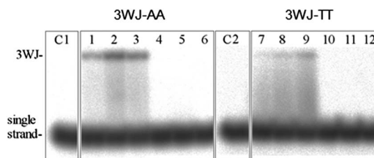
Fig. 10 Autoradiograms of the gels run at room temperature. Lane C1: control containing the three strands, S1-AA, S2 and S3. Lanes 1–3: S1-AA, S2 and S3 mixed with \Delta_{Fe}/S_C-[Fe_2L^{1a}_3]Cl_4 at 0.5 : 1, 1 : 1 and 2 : 1 (flexicate : 3WJ) ratios, respectively. Lanes 4–6: S1-AA, S2 and S3 mixed with \Delta_{Fe}/R_C-[Fe_2L^{1a}_3]Cl_4 at 0.5 : 1, 1 : 1 and 2 : 1 (flexicate : 3WJ) ratios, respectively. Lane C2: control containing the three strands, S1-TT, S2 and S3. Lanes 7–9: S1-TT, S2 and S3 mixed with \Delta_{Fe}/S_C-[Fe_2L^{1a}_3]Cl_4 at 0.5 : 1, 1 : 1 and 2 : 1 (flexicate : 3WJ) ratios, respectively. Lanes 10–12: S1-TT, S2 and S3 mixed with \Delta_{Fe}/R_C-[Fe_2L^{1a}_3]Cl_4 at 0.5 : 1, 1 : 1 and 2 : 1 (flexicate : 3WJ) ratios, respectively.
