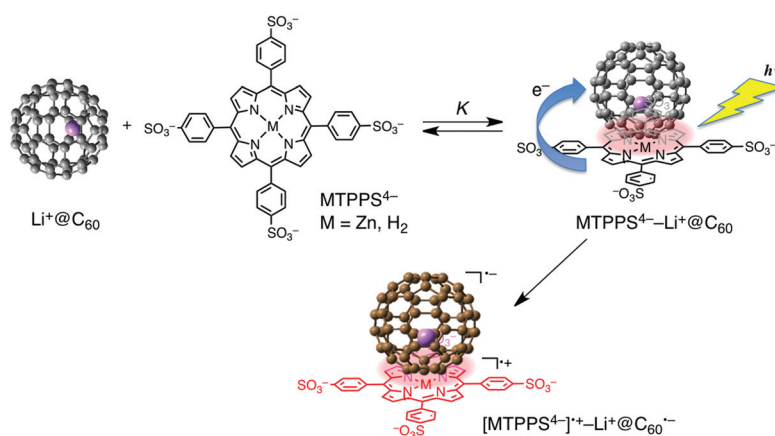
Scheme 1 Supramolecular complex formation and photoinduced charge separation of \text{MTPPS}^{4-} (M = Zn and H 2 ) with \text{Li}^+\text{@C}_{60} in PhCN.
