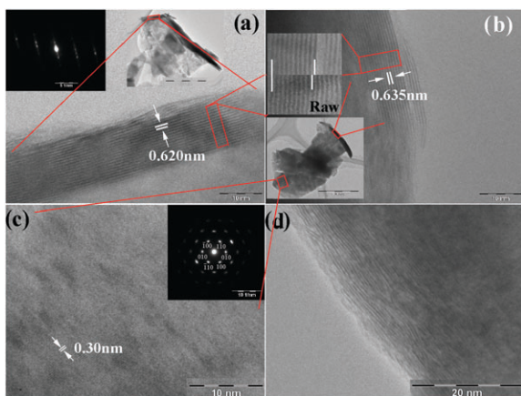
Fig. 1 Transmission electron microscope (TEM) images of raw and restacked MoS 2 : (a) raw MoS 2 , with the inset showing the corresponding SAED pattern; (b) restacked MoS 2 , with the top inset showing a direct comparison of the layer spacing of raw and restacked MoS 2 by a comparison of 9 layers, while the bottom inset indicates the particle source of the images enlarged in (b) and (c); (c) restacked MoS 2 , with the inset showing the corresponding SAED pattern; (d) turbostratically restacked MoS 2 .
